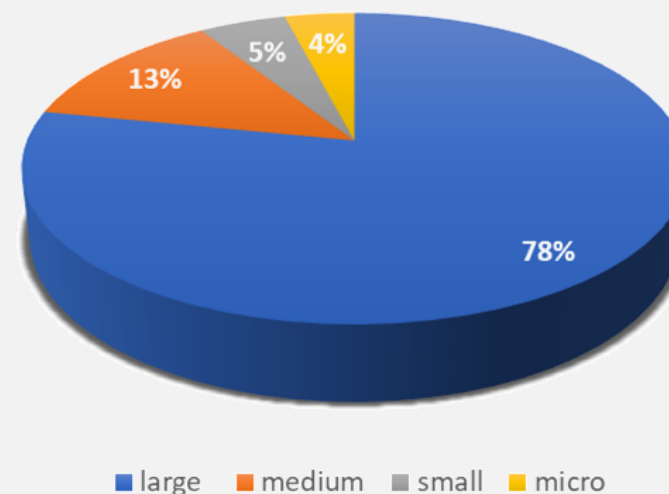
Dataset composition
